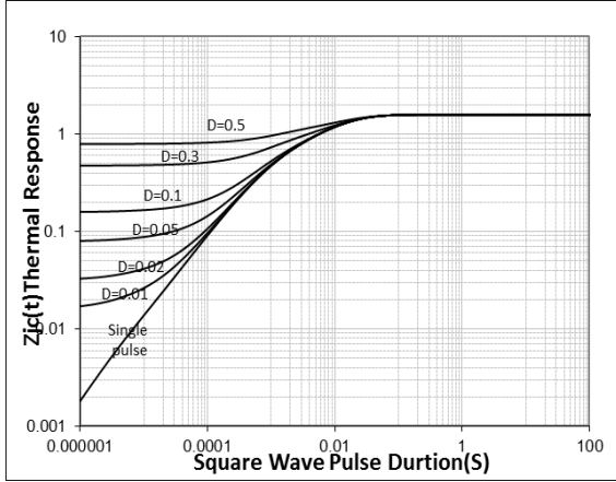
Transient Thermal Response Curve For MS65R620R/DPAK
