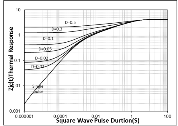
Transient Thermal Response Curve For MS65R620R/TO-220MF-K1
