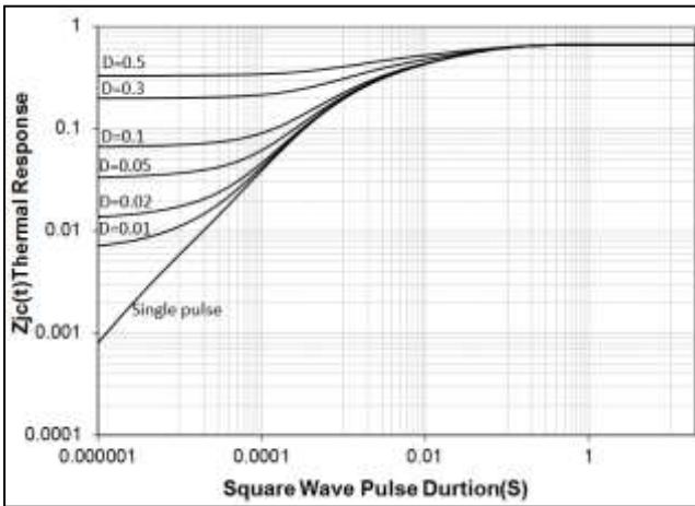
Normalized Maximum Transient Thermal Impedance for IGBT(RJC)-TO-247
