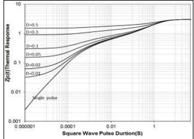
Normalized Maximum Transient Thermal Impedance for IGBT(RJC)-TO-220MF
