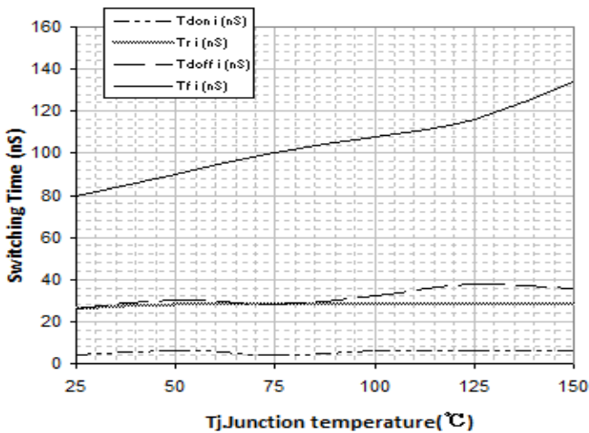
Switching Time vs. Tj
